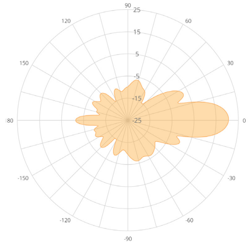
C5 Azimuth Polar Plot
